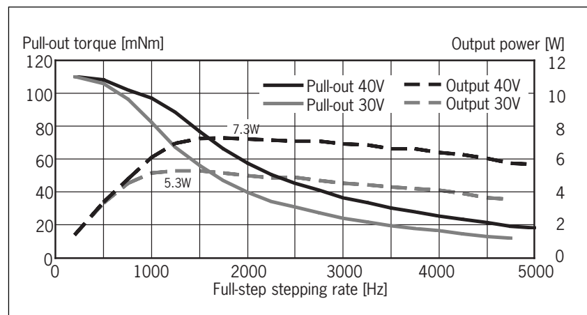
Figure 13. Performance as a function of chopper voltage for a 25ohm bipolar 42mm square hybrid stepper driven by PBL3770A constant-current driver (Chopper voltage 40/30V, winding current 280mA).
